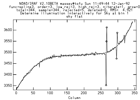
Figure 25: The fit along the spatial axis to the twilight sky exposure that has been “flattened” by the normalized dome-flat.
